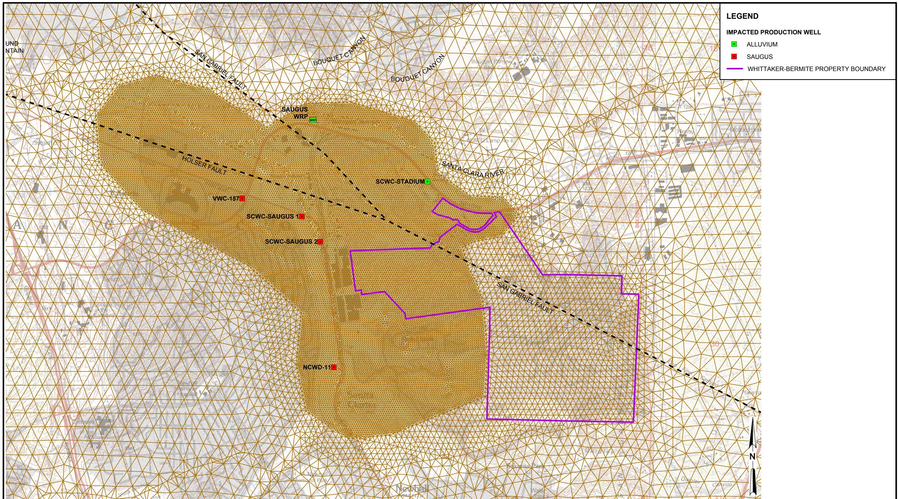
FIGURE 2-6 LOCAL MODEL GRID ANALYSIS OF PERCHLORATE CONTAINMENT IN GROUNDWATER NEAR THE WHITTAKER-BERMITE PROPERTY SANTA CLARITA, CALIFORNIA
