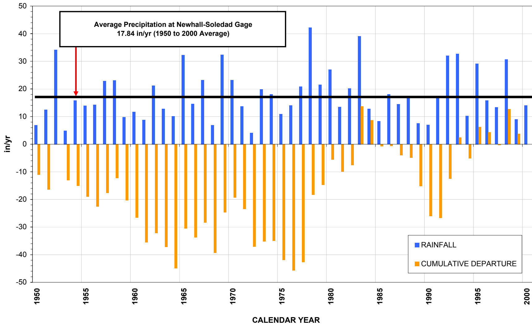
FIGURE 2-8 ANNUAL PRECIPITATION AND CUMULATIVE DEPARTURE FROM THE 1950 THROUGH 2000 AVERAGE AT THE NEWHALL-SOLEDAD RAIN GAGE
