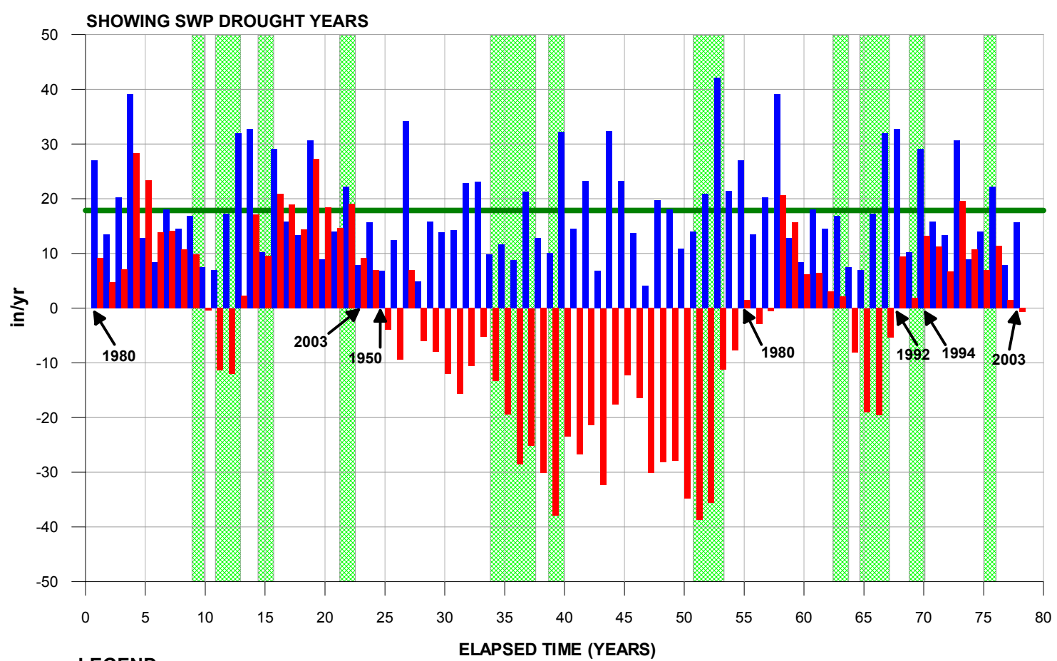
FIGURE 2-9 ANNUAL PRECIPITATION AND CUMULATIVE DEPARTURE FROM THE 1950 THROUGH 2000 AVERAGE AT THE NEWHALL-SOLEDAD RAIN GAGE FOR THE 78-YEAR SIMULATION PERIOD ANALYSIS OF PERCHLORATE CONTAMINATION IN GROUNDWATER NEAR THE WHITTAKER-BERMITE PROPERTY SANTA CLARITA, CALIFORNIA
