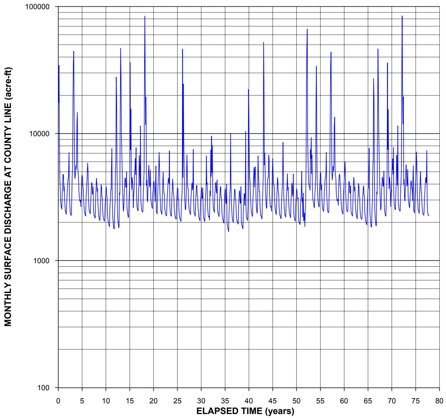
FIGURE 2-17 SIMULATED SANTA CLARA RIVER FLOW AT COUNTY LINE ANALYSIS OF PERCHLORATE CONTAINMENT IN GROUNDWATER NEAR THE WHITTAKER-BERMITE PROPERTY SANTA CLARITA, CALIFORNIA
